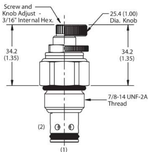
Screw/Knob Version
