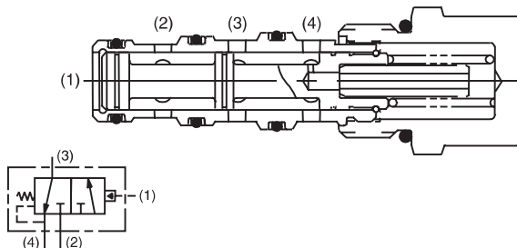
"B" SPOOL — DH103B
