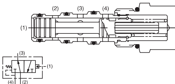
"C" SPOOL — DH103C
