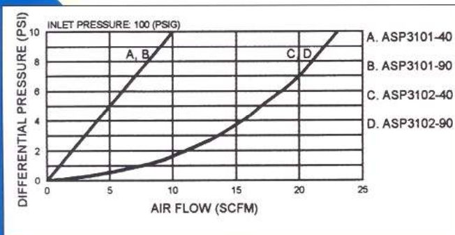
ASP3101 & ASP3102 Differential Pressure vs. Air Flow
