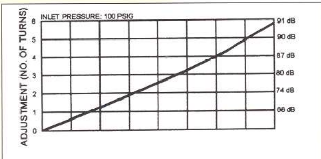
ASP-3SC & ASP-2SCH Adjustment vs. dB Rating
