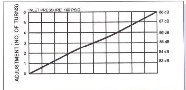
ASP-8SC Adjustment vs. dB Rating
