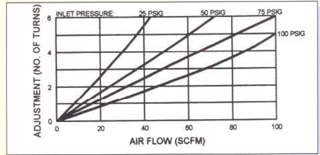
ASP-8SC Adjustment vs. Air Flow
