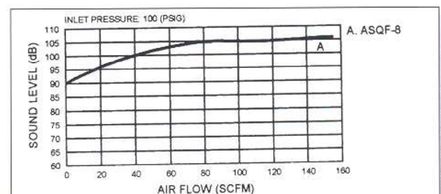
ASQF-8 dB Rating vs. Air Flow
