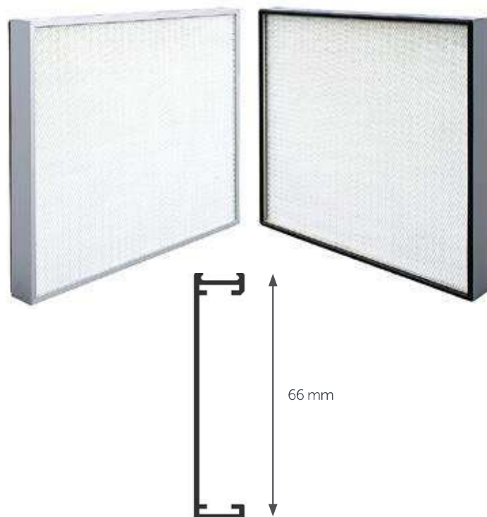
66 mm Aluminium Profile View
