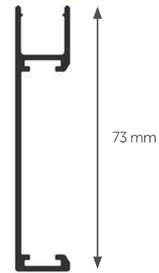
73 mm Aluminium Profile View
